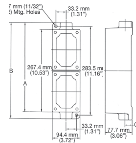
Tandem Mounting Box
