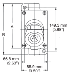
Single Gang Mounting Box with Receptacle Cover
