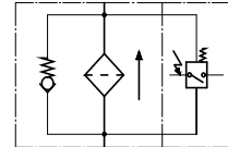
filter with electrical clogging indicator
