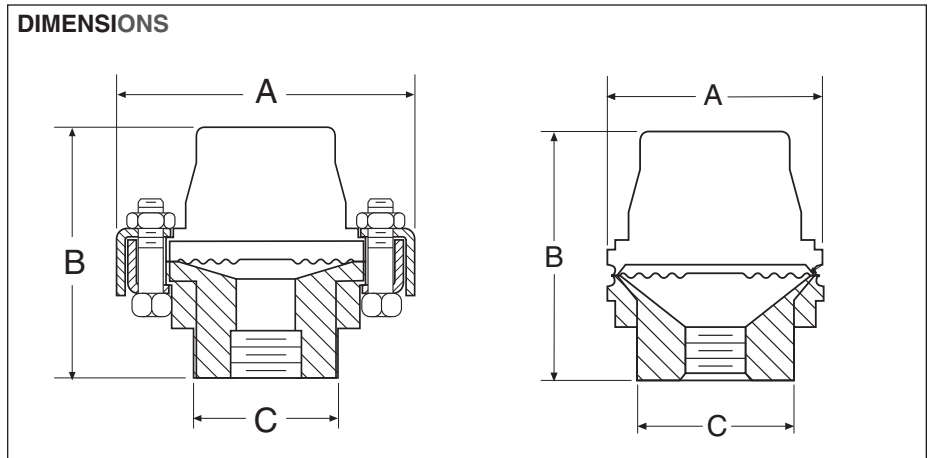
Type 400 Threaded
